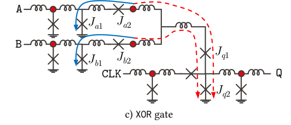
Figure 4: Asynchronous input, synchronous output (AS) components. The solid blue and dashed red lines denote the storage loops in, respectively, logical 0 and 1 state.
